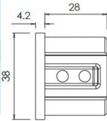
38mm End Cap for Glass Top Rail
