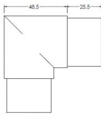
38mm 90 Degree Joiner for Glass Offset Rail
