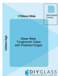
1750 x 1200mm Glass Pool Fence or Balustrade Panel
