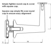
50 x 50mm cap
