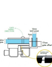
Glass Gate Latch for Internal Glass to Glass
