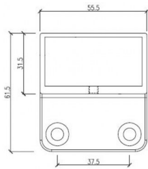
50x25mm Wall Plate for Glass Offset Rail
