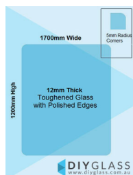
1700 x 1200mm Glass Pool Fence or Balustrade Panel
