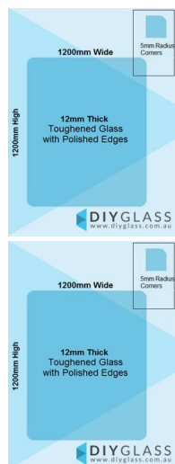
1200 x 1200mm Glass Pool Fence or Balustrade Panel
